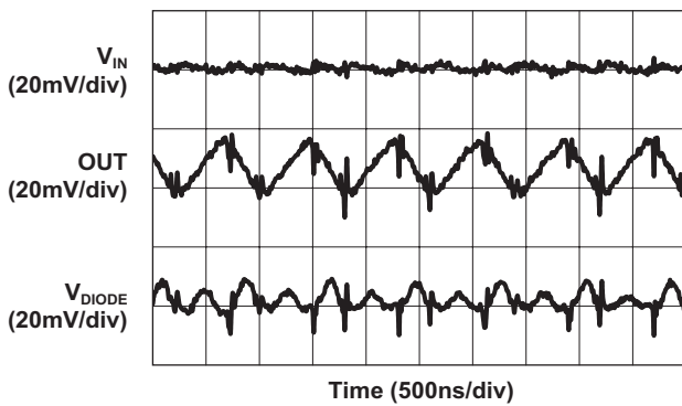
60mA Load Characteristics
