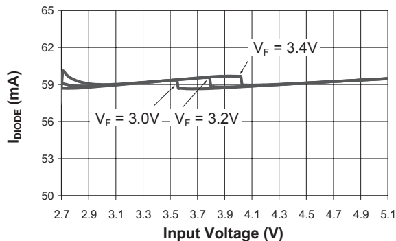
I_{DIODE} vs. Input Voltage (3x20mA)
