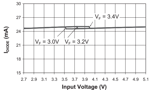
I_{DIODE} vs. Input Voltage (3x8.3mA)
