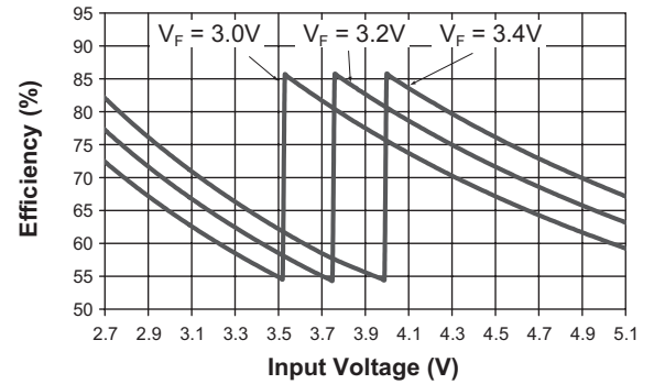
Efficiency vs. Input Voltage (3x8.3mA)
